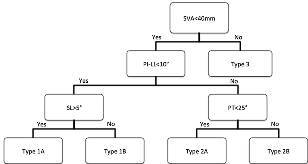
Fig. 4 Decision-tree algorithm
